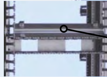
Horizontal managers with removable door that hinges top or bottom, allows for easy cable access. Flips up, stays up.
