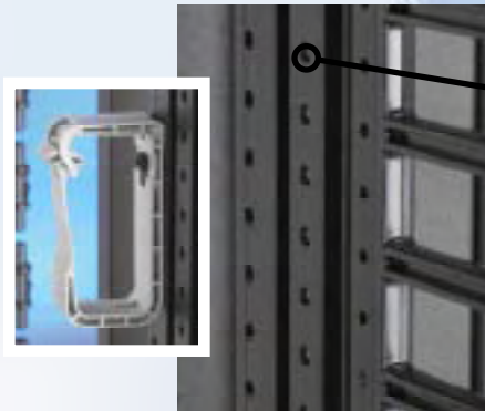
Accessory mounting holes run the full length of all vertical sections to accommodate attachment of dozens of cable management accessories.
